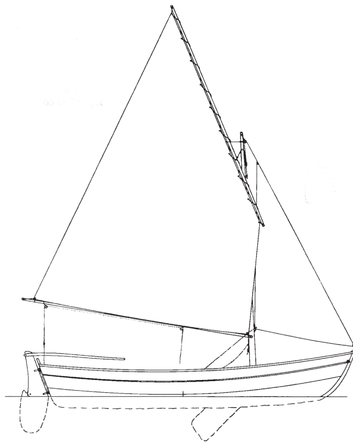
Joel White's Pooduck courtesy of WoodenBoat Publications
